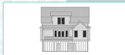
Rear Elevation
